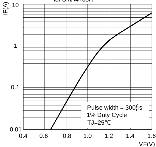
FIG4: Typical Instantaneous Forward Characteristics for SMA4763A
