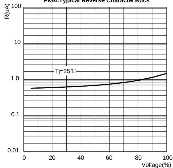
图4: 反向电流曲线 FIG4: Typical Reverse Characteristics
