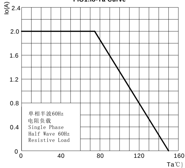
图1: I_o - T_a 曲线 FIG1: I_o - T_a Curve
