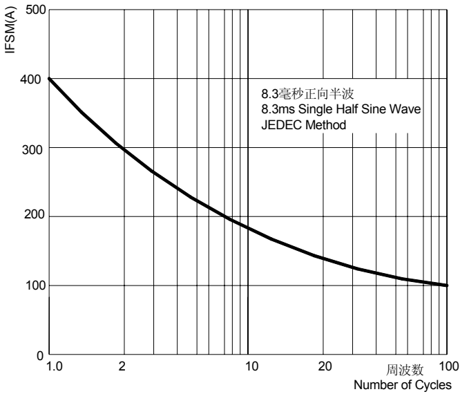
图2：最大正向浪涌冲击耐受力 FIG.2: MAXIMUM NON-REPETITIVE FORWARD SURGE CURRENT
